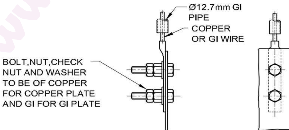
ENLARGED DETAIL 'A'
